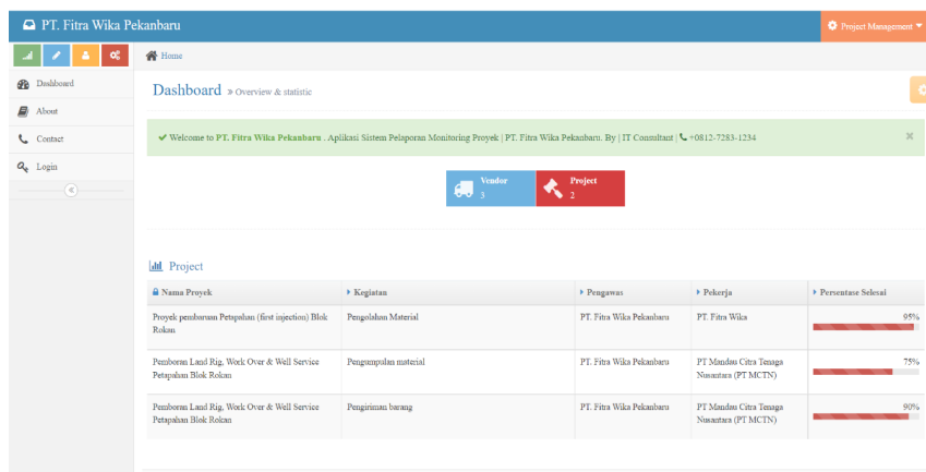
Figure 5. Home Page
