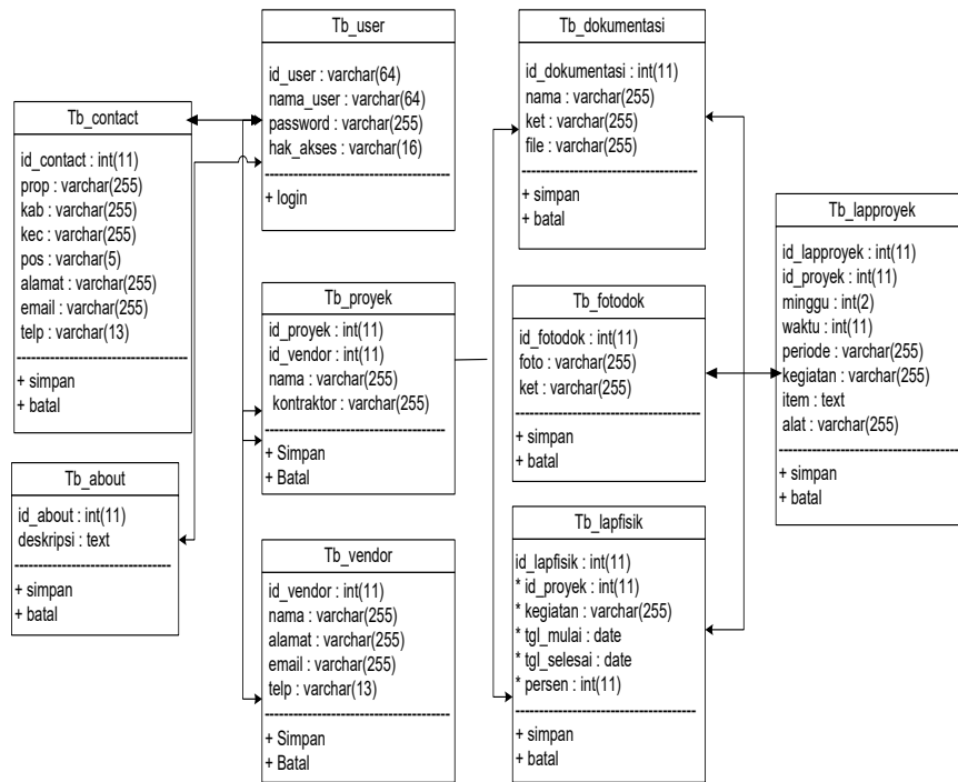
Figure 3. Class Diagram
