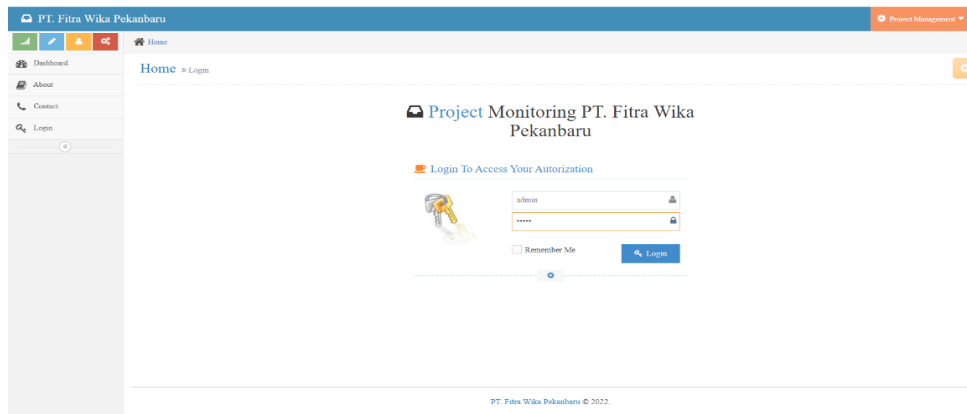
Figure 3. Login Page
