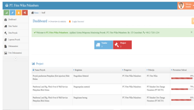
Figure 6. Staff Page
